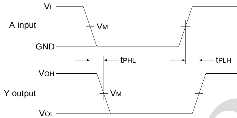
Figure 4. The input A to output Y propagation delays
