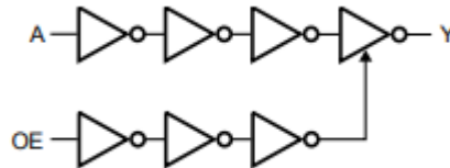
Figure 2. Logic diagram
