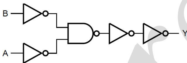
Figure 2. Logic diagram
