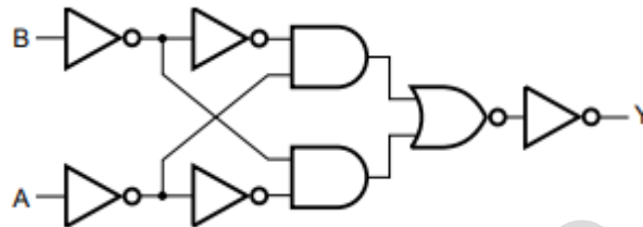
Figure 2. Logic diagram
