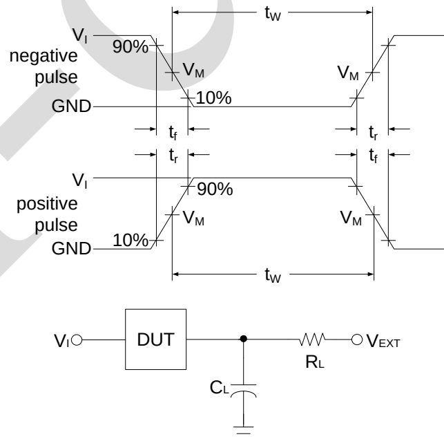
Figure 3. Test circuit for measuring switching time
