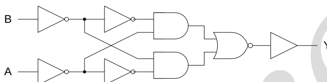
Figure 2. Logic diagram
